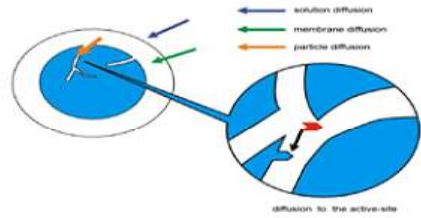
schematic diagram of the adsorption process
